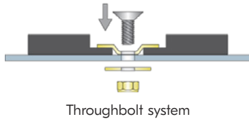
Throughbolt system
