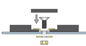
Throughbolt system
