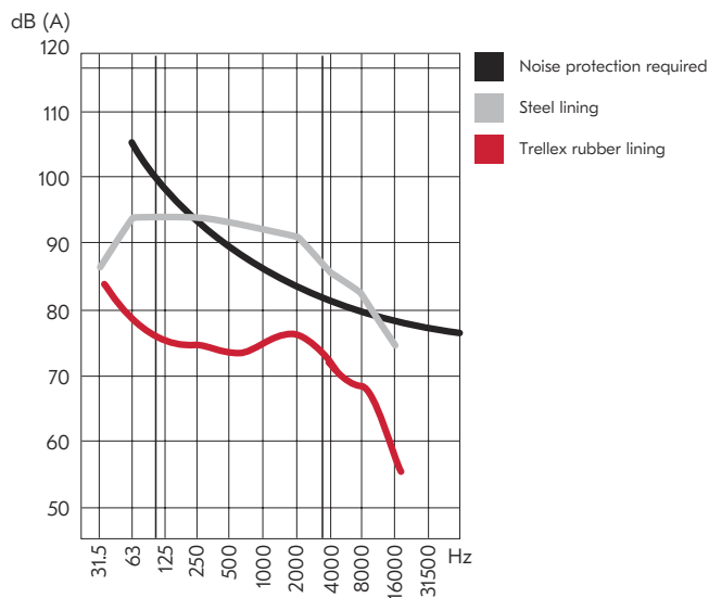
Diagram sound level - Loading truck
