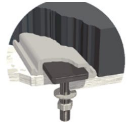
T-bolt fixing system
